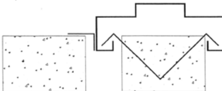
Cavity wall application using B146 profile with 30x19 weather mould.
